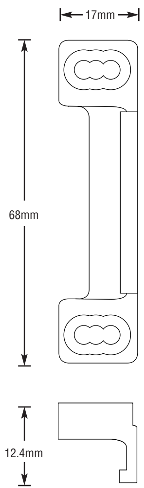
17mm Stack Height 94200
